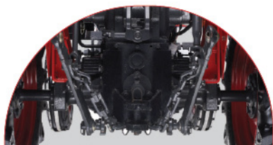
Extra pin in 3 point linkage for lower link mounting To reduce lipping on soft soils.
